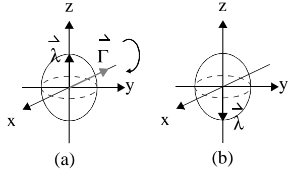
FIGURE 2. NOT operation. (a) The initial state is \hat{\lambda}=(0,0,+1) or P=-1 . (b) The final state obtained after 180^\circ rotation around the x axis in the negative direction is \hat{\lambda}=(0,0,-1) or P=+1 .
